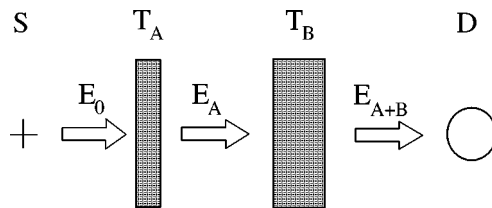
Figure 16. Set-up of a nuclear target consisting of two parts; T_A and T_B are the effective resonance thicknesses of the constituent targets, S and D are source and detector, E_0 represents the source radiation field, E_A and E_{A+B} represent the transmitted fields.
