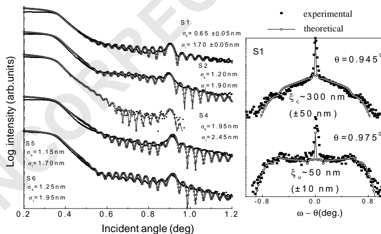
Fig. 1. XRR scans of [Fe(3.0 nm)/Tb(2.0 nm)] ×20 multilayers along with their fit deposited on FG substrates with different etching times. The substrate roughness ( \sigma_s ) and interface roughness ( \sigma_i ) are shown. The inset shows the transverse ( \omega ) scan for S1 along with the fit at two different angles of \theta corresponding to the position at the Bragg peak and at an off-set to it. At \omega - \theta the specular peak is seen over a diffuse background. For clarity, various curves are shifted relative to each other along the y-axis.
