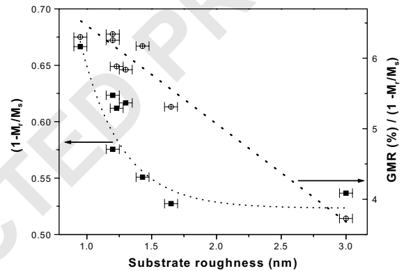
Fig. 3. The change in AFF (■) with increase in substrate roughness as obtained from SQUID measurements. Also shown is the GMR normalised to AFF ( \oplus ) with increasing roughness.
