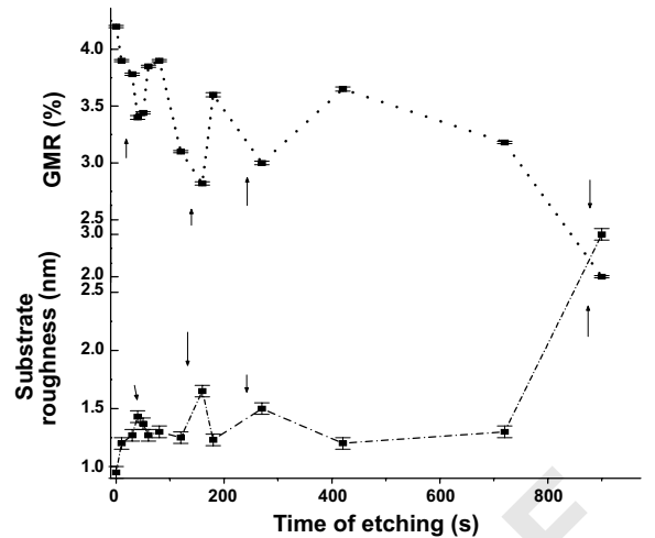
Fig. 2. The plot of surface roughness of the FG substrates and the corresponding GMR ratio as obtained from the fit to the XRR data and the magnetoresistance measured. The arrows indicate the points for variation maximum/minimum in roughness/GMR.
