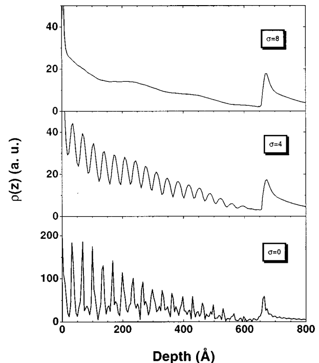
FIG. 6. Fourier transform as indicated in Eq. (4) where R(q) has been obtained by simulation of a [33 Cu/33 Co] 10 multilayer with three different interface roughnesses.
