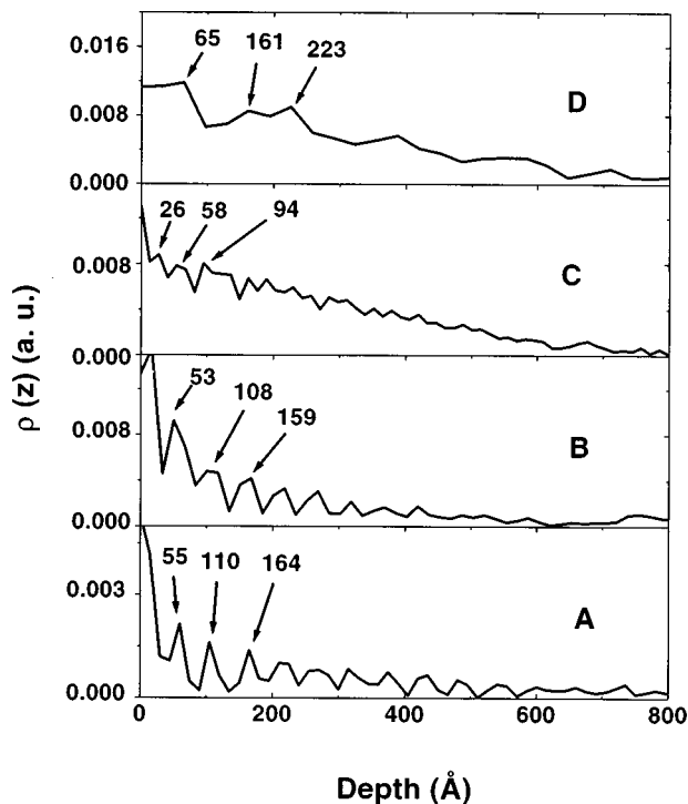
FIG. 7. Fourier transform as indicated in Eq. (4) of the experimental reflectivity. (a) Data obtained for (50 Co/50 Cu) 7 at incident energy of 7704 eV. (b) The same sample at 8052 eV. (c) Data obtained for (33 Co/33 Cu) 10 at incident energy of 7704 eV. (d) The same sample at 8052 eV.
