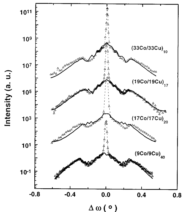
FIG. 3. Rocking curves taken at constant values of 2\theta placed at a Kiessig maximum around 2\theta_M=1.32^\circ . For the sake of clarity \Delta\omega=\omega-\theta_M has been taken as the variable. The fits to the experimental patterns are based on the DWBA. The specular peak has not been reproduced in the simulations.
