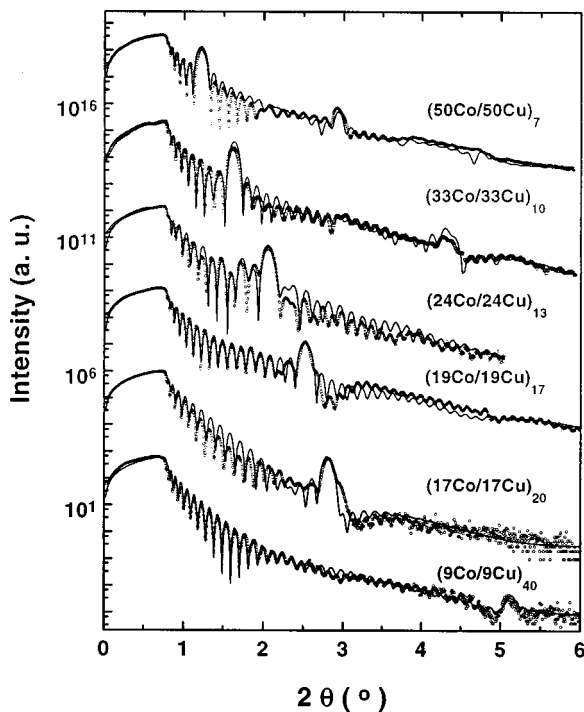
FIG. 2. Specular reflectivity patterns of Co/Cu multilayers recorded at an incident energy just under the Co absorption K edge (7704 eV). Points correspond to the experimental patterns and solid lines have been calculated by the simulation program.
