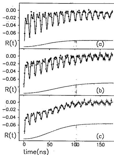
FIG. 4. PAC time spectra taken on \text{MgO}/[\text{Fe}(3.0 \text{ nm})/\text{Cr}(t_{\text{Cr}})]_{10} multilayers with Cr thickness up to 5.1 nm, obtained at 293 K in the in-plane geometry. The Cr thicknesses are (a) 0.9 nm, (b) 3.3 nm, and (c) 5.1 nm. The dashed lines represent the chromium contribution.
