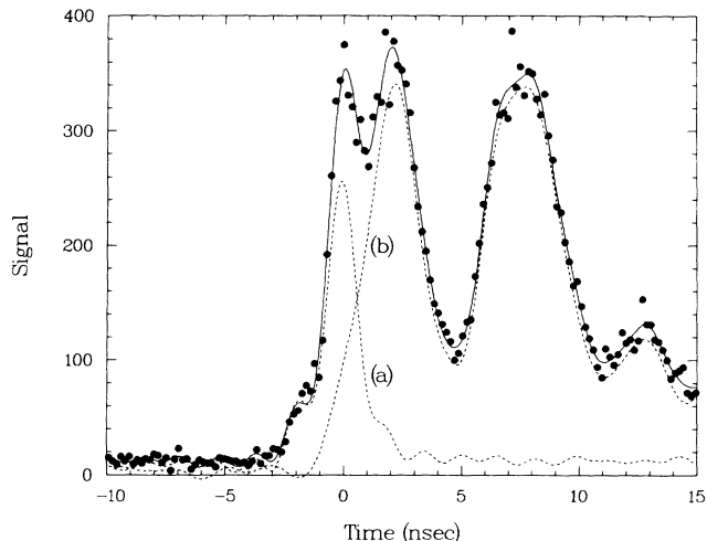
FIG. 2. The first 15 nsec of the time spectrum is shown, together with its smoothed curve. The broken curves are (a) the Fourier smoothed off-resonance spectrum and (b) the result of the subtraction of this spectrum from the smoothed resonant spectrum.
