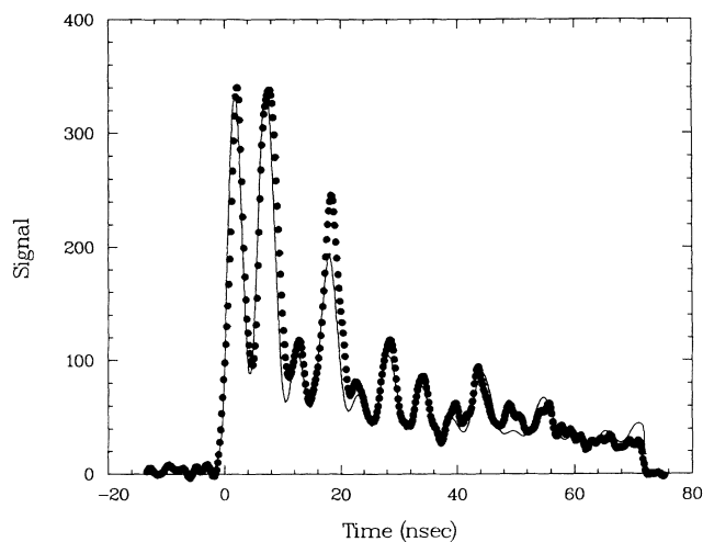
FIG. 3. The smoothed experimental data with its prompt background removed is compared with a dynamical diffraction calculation (continuous curve) described in the text.
