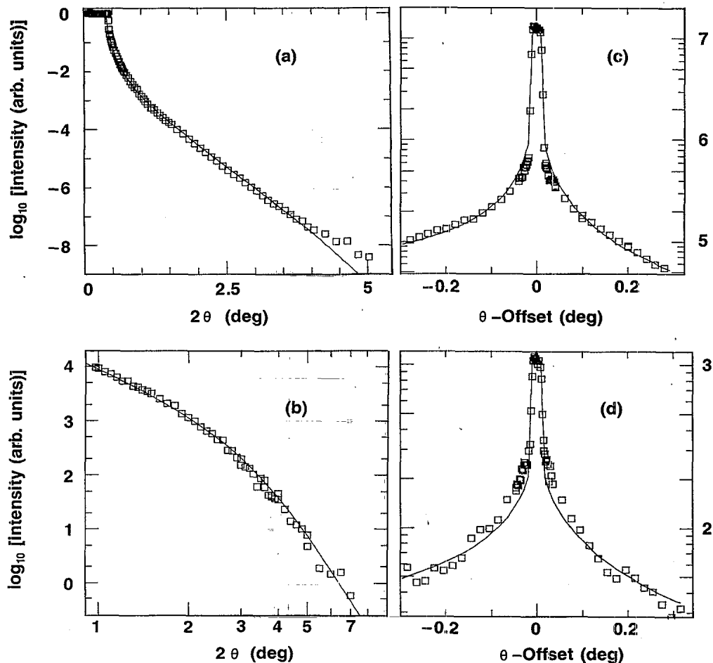
FIG. 7. Measured x-ray intensity vs angle for polished Pyrex surface. Data is represented by squares and fits by solid lines. Statistical errors are approximately the size of the squares. Intensities are on arbitrary logarithmic scales. Fits yielded the parameters \sigma = 7.6 \text{ \AA} , \xi = 7000 \text{ \AA} , and h = 0.2 . (a) Specular reflection with diffuse subtracted out. (b) Diffuse scattering near specular \theta_1 = \theta_2 + 0.03^\circ . ( 2\theta is a log scale.) (c), (d) Transverse (rocking) scans; diffuse and specular are convolved with resolution. Intensity vs \theta offset ( \theta_1 - \theta_2 ) at (c) 2\theta = 2^\circ and (d) 2\theta = 4^\circ . The systematic discrepancies between the fits and the data show that the roughness of this polished glass is not exactly given by the simple expression used.
