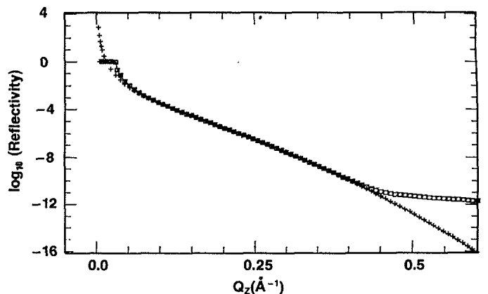
FIG. 5. The computed reflectivity of Pyrex at \lambda = 1.46 \text{ \AA} with \sigma = 8 \text{ \AA} , using the Born approximation (crosses), the DWBA (open squares), and the form given by Eq. (4.34) (solid line).
