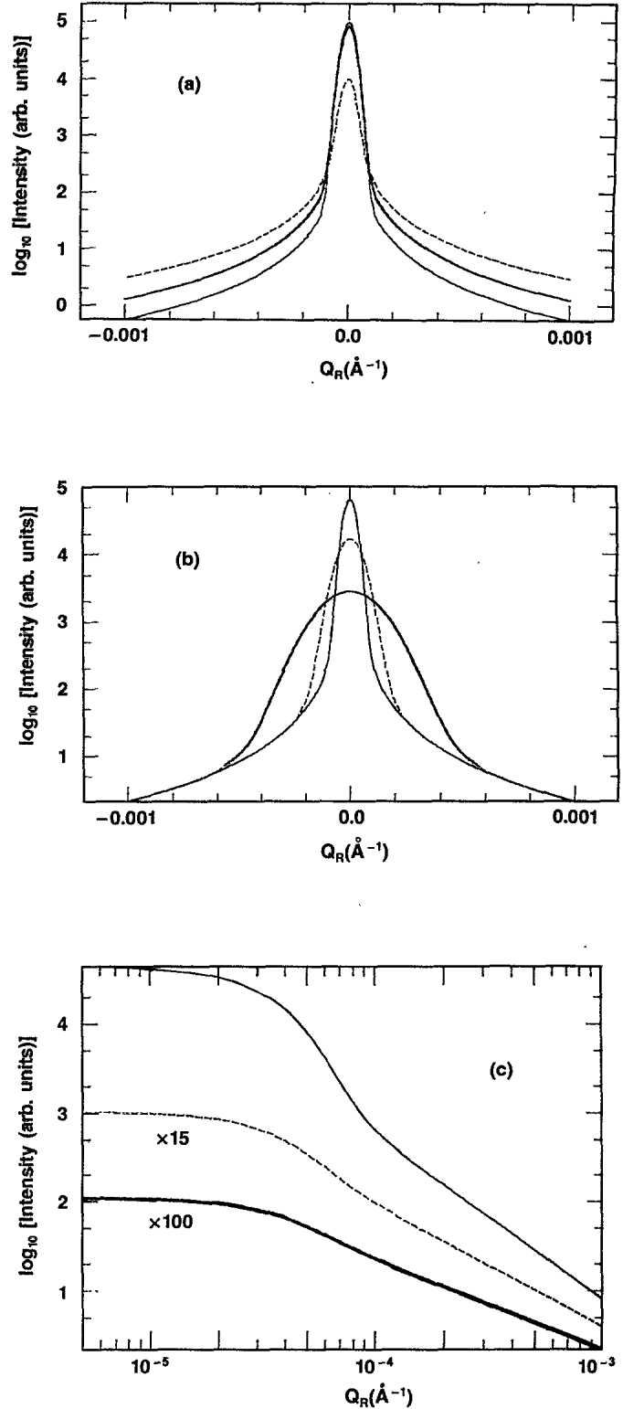
FIG. 3. Calculated intensity vs q_r using Eq. (2.33) with A = 0 . (a) q_z = 0.3 \text{\AA}^{-1} , \xi = 1 \times 10^5 \text{\AA} , B = 0.2 (solid line), B = 0.5 (bold line), B = 5.0 (dashed line). Note the variation in peak-to-tail ratio. (b) q_z = 0.3 \text{\AA}^{-1} , B = 1.0 , \xi = 1 \times 10^5 \text{\AA} (solid line), \xi = 5 \times 10^4 \text{\AA} (dashed line), \xi = 2 \times 10^4 \text{\AA} (bold line). Note the variation in the central peak width. (c) log-log plot showing the different values for the limiting slope where B = 8 , \xi = 1 \times 10^5 \text{\AA} , q_z = 0.2 \text{\AA}^{-1} \eta = 0.16 (solid line), q_z = 0.4 \text{\AA}^{-1} \eta = 0.64 (dashed line) (scaled \times 15 ), q_z = 0.5 \text{\AA}^{-1} \eta = 1.0 (bold line) (scaled \times 100 ).
