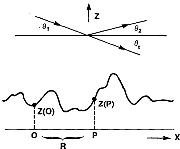
FIG. 1. Schematic of a rough surface. z is the normal to the surface. x is along the average surface in the specular scattering plane. \theta_1 is the grazing angle of incidence, \theta_2 is the grazing angle of reflection, and \theta_t is the grazing angle of refraction. z(P) is the height of the surface at point P . At specular \theta_1 = \theta_2 .
