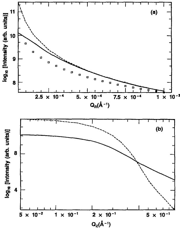
FIG. 2. Calculated S_{\text{diff}}(q) as calculated from the equations given in the text. (a) S(q) vs q_r (in \text{\AA}^{-1} ) for q_z = 0.01 \text{\AA}^{-1} . Solid line represents the case where h = 0.5 , \sigma = 7 \text{\AA} , \xi = 7000 \text{\AA} ; dashed line represents the case with no cutoff; open squares represent the case where h = 0.2 , \sigma = 7 \text{\AA} , \xi = 7000 \text{\AA} . (b) S(q) vs q_z (in \text{\AA}^{-1} ). Solid line represents case where h = 0.5 , \sigma = 7 \text{\AA} , \xi = 7000 \text{\AA} ; dashed line represents case where h = 0.2 , \sigma = 7 \text{\AA} , \xi = 7000 \text{\AA} . For longitudinal ( q_z ) scans, the shape of S(q) is unaffected by \xi .
