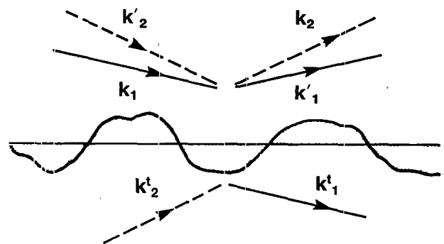
FIG. 4. Schematic of a rough surface. The horizontal line is the average surface ( z=0 ). The shaded regions are the regions of perturbation to a smooth surface. The incident wave vectors k_1 and -k_2 , the reflected wave vectors k_1' and -k_2' , and the transmitted wave vectors k_1'' and -k_2'' are illustrated.
