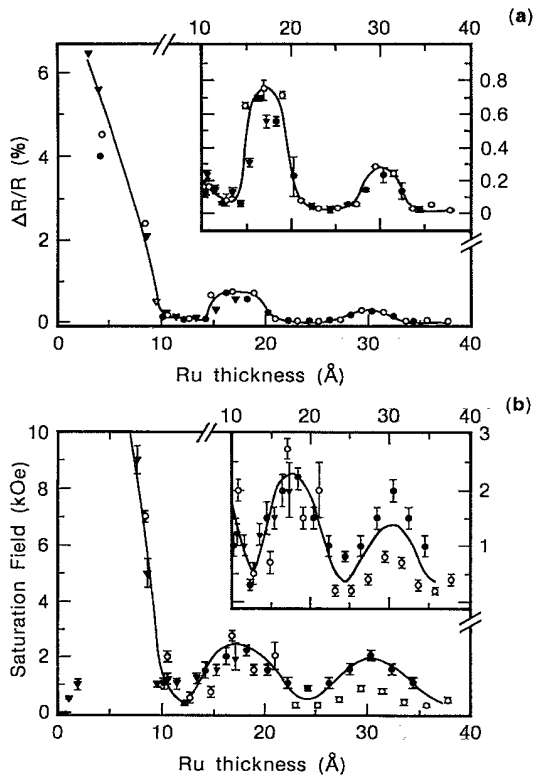
FIG. 3. (a) Transverse saturation magnetoresistance (4.5 K) and (b) saturation field (300 K) vs Ru layer thickness for structures of the form Si(111)/(100 Å) Ru/(20 Å) Co/ t_{Ru} Ru/20/(50 Å) Ru deposited at temperatures of ●, 40°C; ○, 125°C; ×, 200°C.
