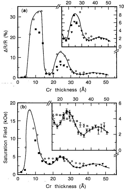
FIG. 4. (a) Transverse saturation magnetoresistance (4.5 K) and (b) saturation field (4.5 K) vs Cr layer thickness for three series of structures of the form Si(111)/(100 Å) Cr/(20 Å) Fe/ t_{Cr} Cr/ N /(50 Å) Cr, deposited at temperatures of Δ, ■, 40°C ( N=30 ); ○, 125°C ( N=20 ).
