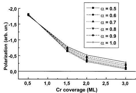
Fig. 2. Coverage dependence of polarisation on Cr atoms for Cr overlayer on Fe with ‘smooth’ interface generated by ‘epitaxy’ (interface region is 10–11 layers). Different symbols correspond to various values of the parameter \alpha .
