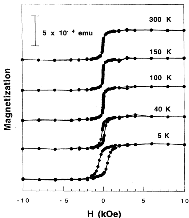
FIG. 1. Magnetization as a function of applied field H for two 14.3-Å equivalent thickness Fe deposits grown on MgO(001) at 700 K and separated and capped by 200-Å MgO deposits. Hysteretic behavior develops at the lower temperatures.
