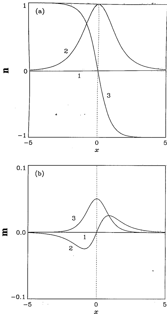
FIG. 2. A static AFM domain wall illustrated through the three components of (a) the vector \mathbf{n} = (n_1, n_2, n_3) and (b) the magnetization density \mathbf{m} = (m_1, m_2, m_3) . Dashed lines correspond to the results of a numerical calculation in the discrete spin model with \epsilon = 0.1 but are difficult to distinguish from the solid lines depicting the continuum solution [(2.15) and (2.16)].
