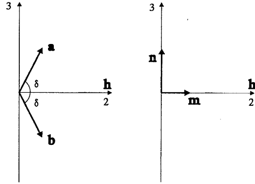
FIG. 5. Schematic illustration of a canted AFM state for an applied in-plane field \mathbf{h} = (0, h, 0) . The two spins tilt toward the magnetic field each at an angle \delta given by Eq. (4.13).
