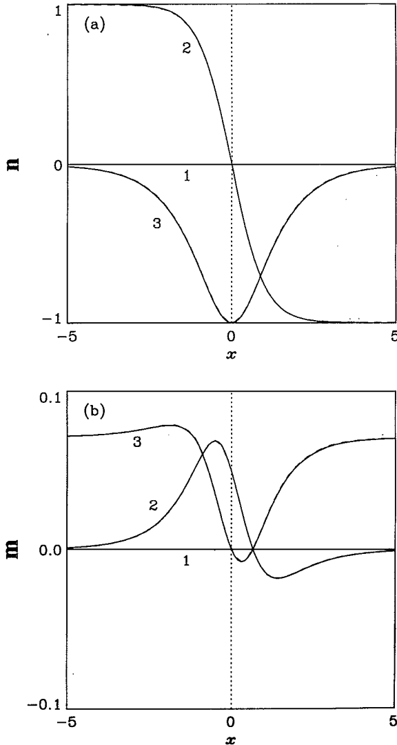
FIG. 7. A static AFM domain wall in the presence of a field applied along the easy axis; \mathbf{h} = (0, 0, h) with h > 1 . Dashed lines correspond to a numerical calculation with \varepsilon = 0.1 and h = \sqrt{2} but are indistinguishable from the solid lines depicting the continuum solution [(4.24) and (4.25)].
