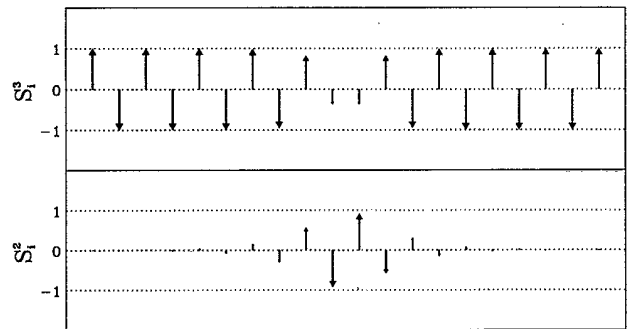
FIG. 1. A static AFM domain wall illustrated through the spin components S_i^1=0 , S_i^2 , and S_i^3 at each lattice site i of a limited portion of the lattice around the wall center. The wall is rather narrow due to the large anisotropy used in the corresponding numerical calculation ( \varepsilon=1/2 ).
