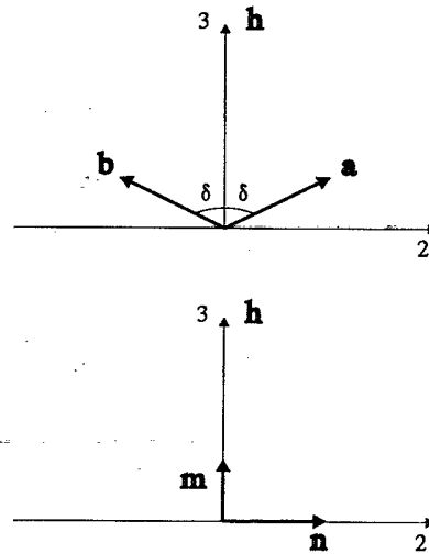
FIG. 6. Schematic illustration of a canted AFM state for a field applied along the easy axis; \mathbf{h} = (0, 0, h) with h > 1 . Each spin forms an angle \delta with the easy axis given by Eq. (4.18).
