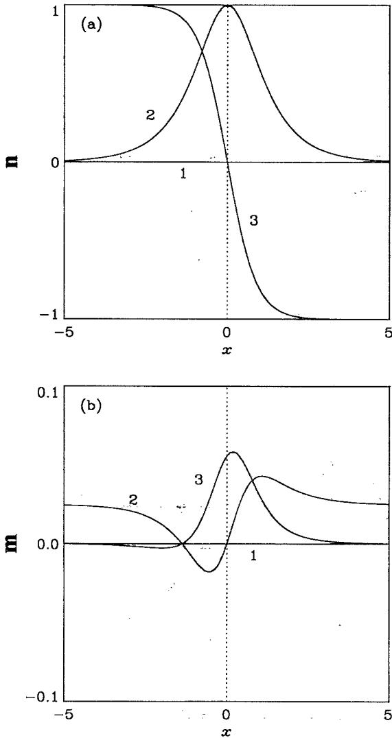
FIG. 4. A static AFM domain wall in the presence of an applied in-plane field \mathbf{h} = (0, h, 0) . Dashed lines correspond to a numerical calculation with \epsilon = 0.1 and h = 1/2 but are indistinguishable from the solid lines depicting the continuum solution [(4.9) and (4.10)].
