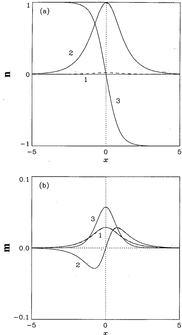
FIG. 3. A moving AFM domain wall illustrated through the vector \mathbf{n} and the magnetization density \mathbf{m} . Solid lines depict the continuum solution [(3.20)–(3.22)] which is found to be in satisfactory agreement with a numerical calculation (dashed lines) for \epsilon = 0.1 and v = 1/2 described in Sec. III.
