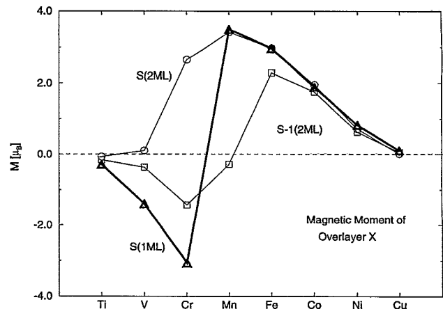
FIG. 1. The magnetic moment for the bcc(100) Fe surface covered by monolayers and bilayers of 3d transition metal X where X = Ti, ..., Cu. The triangles correspond to the magnetic moment of the surface layer, S (1 ML), of the monolayer covered surface. The circles and squares correspond to the surface, S (2 ML), and subsurface, S-1 (2 ML) of the bilayer covered surface.
