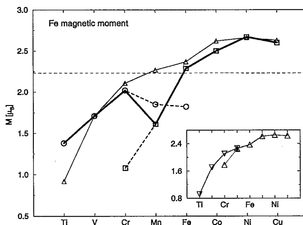
FIG. 2. Calculated magnetic moment of Fe at the interface with X. The bold solid line corresponds to the calculated ground-state moment for the monolayer situation. The broken lines indicate metastable solutions. Circles denote an AFM coupling and squares a FM coupling between the Fe and the overlayer X. The thin line (triangles) corresponds to the Fe interface moment for the bilayer situation. In the inset the Fe interface moment for the bilayer coverage is shown again. The broken line indicates the metastable solutions. Triangles pointing up indicate a FM coupling, triangles pointing down indicate an AFM coupling at the interface.
