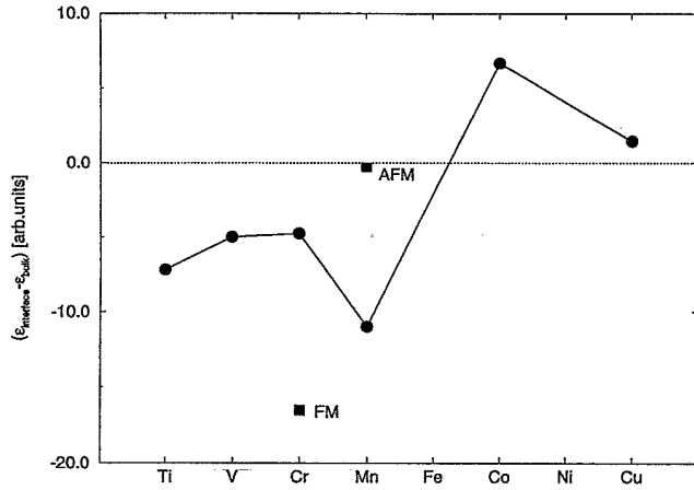
FIG. 3. Calculated exchange coupling of the Fe interface layer according to Eqs. (2)–(4). The solid line corresponds to the calculated ground state, the squares indicate metastable solutions.
