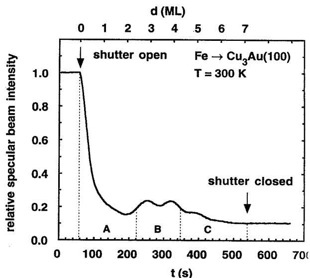
FIG. 1. Intensity variation of the MEED specular beam during the growth of \text{Fe}/\text{Cu}_3\text{Au}(001) at room temperature. The labels A, B, and C distinguish regions of different growth behavior.
