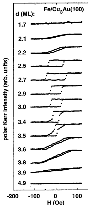
FIG. 2. Hysteresis loops in the polar Kerr effect for various Fe coverages taken at T=160 K. The film thickness ranges from 1.7 to 4.9 ML.
