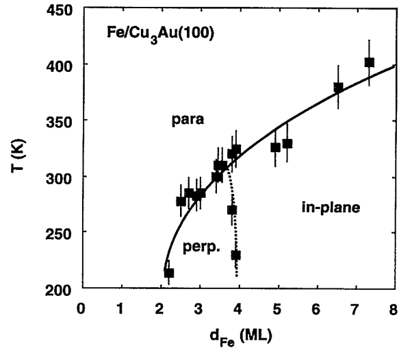
FIG. 4. Magnetic phase diagram of Fe/Cu 3 Au(001). The solid line gives the Curie temperature of the films, whereas the broken line separates the regimes of in-plane and perpendicular magnetization. Both lines serve as a guide to the eye.
