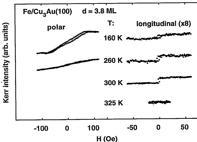
FIG. 5. Temperature dependence of the hysteresis loops in the longitudinal and polar Kerr geometry for a 3.8-ML iron film.
