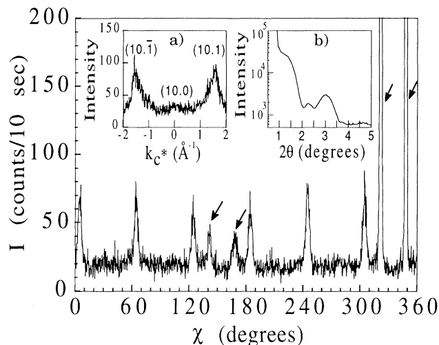
FIG. 1. X-ray \chi scan for [20 \text{ \AA} \text{ Co}/4 \text{ \AA} \text{ Cr}]_{42} superlattice, showing diffraction peaks with 60^\circ symmetry. Inset (a): x-ray c^* scan indicating hcp stacking of Co layers. Inset (b): low-angle x-ray scan showing superlattice peaks. Arrows indicate GaAs (113) and (420) peaks.
