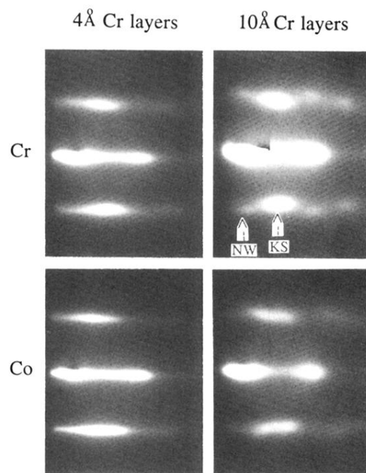
FIG. 2. Representative RHEED images along the \text{Co}\langle 110 \rangle direction. Sharp RHEED streaks are seen for the Co and Cr layers of the [20 \text{ \AA} \text{ Co} / 4 \text{ \AA} \text{ Cr}]_{42} superlattice. In contrast, the Co and Cr layers of the [20 \text{ \AA} \text{ Co} / 10 \text{ \AA} \text{ Cr}]_{33} superlattice indicate a structural transition has occurred.
