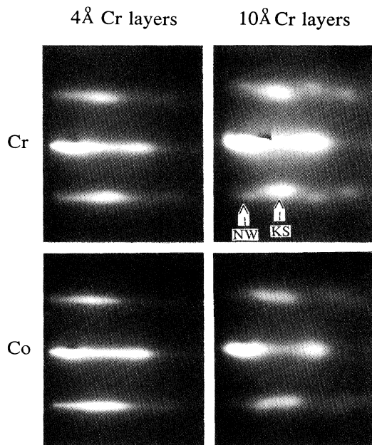
FIG. 2. Representative RHEED images along the \text{Co}\langle 110 \rangle direction. Sharp RHEED streaks are seen for the Co and Cr layers of the [20 \text{ \AA} \text{ Co}/4 \text{ \AA} \text{ Cr}]_{42} superlattice. In contrast, the Co and Cr layers of the [20 \text{ \AA} \text{ Co}/10 \text{ \AA} \text{ Cr}]_{33} superlattice indicate a structural transition has occurred.
