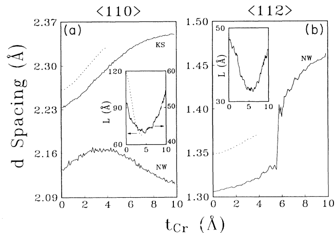
FIG. 3. (a) d spacing profiles during growth of the Cr layers shown in Fig. 2. The RHEED beam is parallel to \text{Co}\langle 110 \rangle , while the dashed and solid lines refer to the 4 \text{ \AA} and 10 \text{ \AA} Cr layers, respectively. (b) RHEED beam parallel to \text{Co}\langle 112 \rangle . Insets are domain size ( L ) profiles with arrows indicating the appropriate y axis. The x axes are the same scale as in the d spacing plots.
