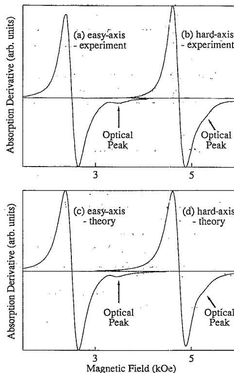
FIG. 4. FMR signal in the sample (\text{Co})_4/(\text{Cu})_6/(\text{Co})_{10.3} along the (a) easy and (b) hard magnetic axes at 36.3 GHz and T=300 K. Note that the optical peaks are weak and occur at higher fields than the acoustic peaks, and therefore the exchange coupling between the Co layers is antiferromagnetic. Note also that the optical peak along the hard axis lies closer to its acoustic counterpart than that along the easy axis. This shows that the exchange coupling is stronger along the easy axis. (c) and (d) are the calculated FMR lines using the theory of the exchange-coupled bilayers for the sample which measurements are shown in (a) and (b). The magnetic parameters for the 4 ML (A) and 10.3 ML (B) of Co(001) films were determined by fitting the positions and intensities of both the acoustic and optical peaks. The best fits were obtained by using the following parameters: (2K_{\parallel}^{\text{eff}}/M_s)^A = -1.22 kOe, (2K_{\parallel}^{\text{eff}}/M_s)^B = -1.18 kOe, (4\pi M_{\text{eff}})^A = 37.3 kOe, and (4\pi M_{\text{eff}})^B = 34.2 kOe (see Table IV). The exchange coupling along the easy axis, J_{\text{easy}} = -0.052 ergs/cm 2 , is higher than that observed for the hard axis, J_{\text{hard}} = -0.025 ergs/cm 2 .
