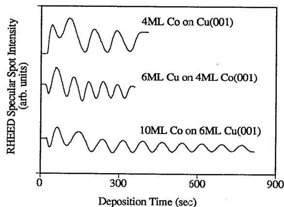
FIG. 2. RHEED intensity oscillations observed during the growth of the Cu/(Co) 4 /(Cu) 6 /(Co) 10.3 /Cu sample. The RHEED intensity was monitored at the specular spot of the RHEED pattern. The electron beam was directed at an angle of 1^\circ with respect to the sample surface. Note that it requires two to three atomic layers to establish regular RHEED oscillation periodicities.
