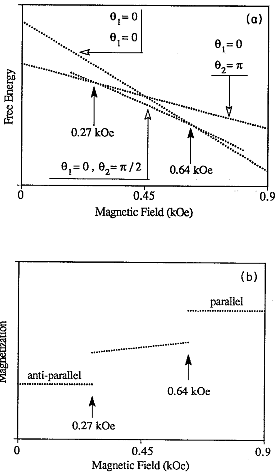
FIG. 9. (a) Magnetic-field dependence of the free energy for a model consisting of a 4-ML Co film exchange coupled with 10-ML Co film. The external field is applied along an easy magnetic axis. The parameters used in the calculation are 4\pi M_s = 17.87 kOe for each film, effective in-plane anisotropy fields 2K_{\parallel}^{\text{eff}}/M_s = -1.10 kOe (4-ML film) and 2K_{\parallel}^{\text{eff}}/M_s = -1.29 kOe (10-ML film), and an angularly dependent antiferromagnetic exchange coupling with J_x = -0.060 ergs/cm 2 and J_1 = 0.015 ergs/cm 2 [see Eq. (12) of the text]. The lowest free energy is obtained for a phase change at 0.64 kOe, where the magnetization in the thin film rotates into the easy-axis direction which is perpendicular to the applied-field direction, followed by a second phase change at 0.27 kOe, where the magnetization in the thin film becomes antiparallel with the magnetization in the thick film. (b) The magnetic-field dependence of the magnetization for the model of (a) assuming that the free energy can reach its minimum value at any applied field.
