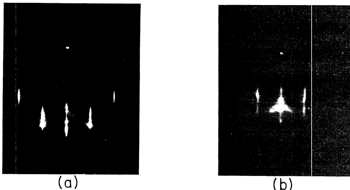
FIG. 1. RHEED patterns corresponding to \{110\} azimuths. (a) Cu(001); (b) 4 ML of Co(001) grown on a Cu(001) substrate.
