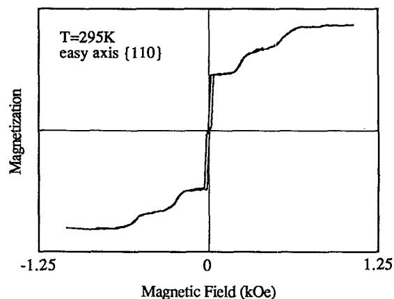
FIG. 8. SMOKE measurements of the hysteresis loop for the sample (\text{Co})_4/(\text{Cu})_{10}/(\text{Co})_{10} . The applied field is applied along the easy magnetic axis. Relatively abrupt changes in the magnetization occur for fields of 0.6 and 0.25 kOe as well as at zero magnetic field. See detailed interpretation in the text.
