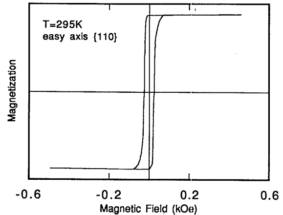
FIG. 10. SMOKE measurement of the hysteresis loop in the sample (\text{Co})_4/(\text{Cu})_6/(\text{Co})_{10} . The applied field is along the easy magnetic axis. Co layers in this sample are coupled antiferromagnetically ( J = -0.052 ) (see Table IV). Note that the hysteresis loop in this sample is square. The fourfold in-plane anisotropy 2K_{\parallel}^{\text{eff}}/M_s \sim 1.2 kOe holds the magnetic moments along the easy axis. No drop in the total magnetic moment was observed at the domain-wall nucleation field 0.5 kOe (corresponding to J = -0.052 ergs/cm 2 ); therefore, this sample does not follow the path of minimum energy.
