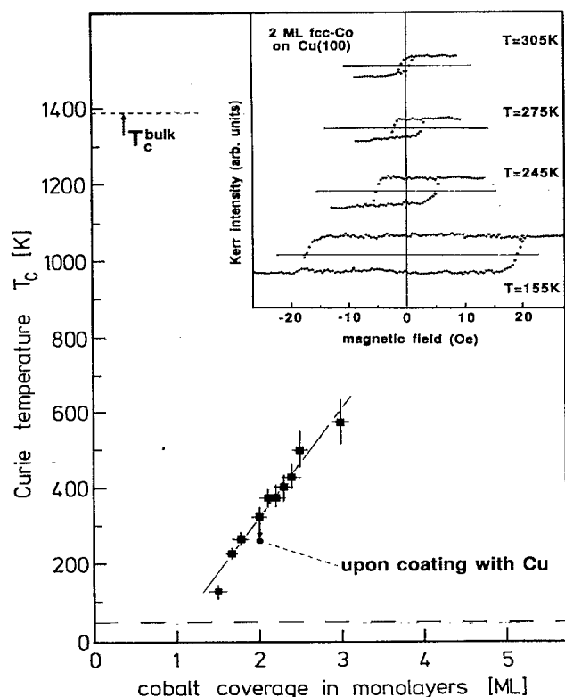
FIG. 1. Coverage dependence of the Curie temperature of fcc-Co films as determined from the SMOKE experiments (the thin line serves to guide the eye). The film thickness in monolayers (ML) has been determined as described in the text. Inset: Variation of the hysteresis loop of a 2-ML film with sample temperature. This temperature dependence has been used to determine T_C(d_{ML}) (see also Ref. 10).
