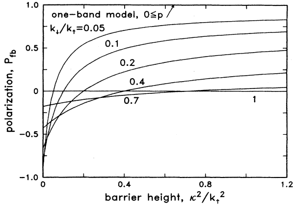
FIG. 3. Effective spin polarization P_{fb} for the magnetic valve effect, Eqs. (3.4) and (3.5). For Fe, Co, Ni and their alloys, the barrier height in eV is about 5 times the abscissa \kappa^2/k_t^2 .
