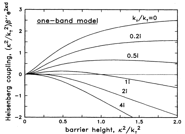
FIG. 4. Reduced Heisenberg-exchange coupling (\kappa^2/k_t^2)b''e^{2\kappa d} vs reduced barrier height in the one-band model, Eq. (4.5).
