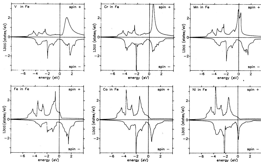
FIG. 1. Local densities of states of 3d impurities in Fe for both spin directions. The figure denoted “Fe in Fe” represents the density of states of pure Fe.
