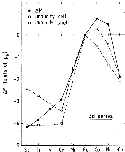
FIG. 9. Contributions to the total change \Delta M of the magnetization ( \bullet ) due to 3d impurities ( \circ , contribution from the impurity cell; \square , sum of the contributions from the impurity cell and first-shell atoms).
