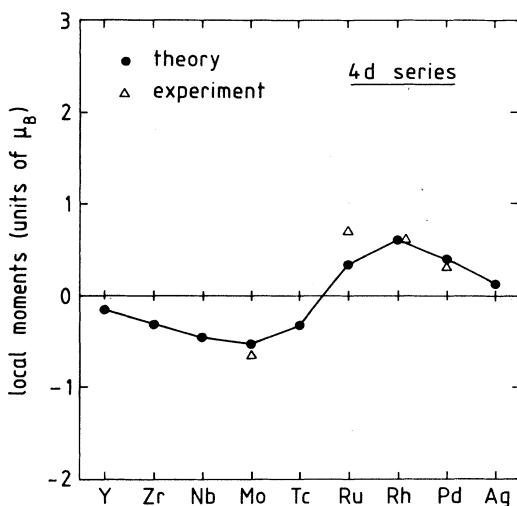
FIG. 5. Local moments in the impurity Wigner-Seitz sphere for 4d impurities in Fe. The triangles are experimental values from neutron scattering (Refs. 29 and 53).
