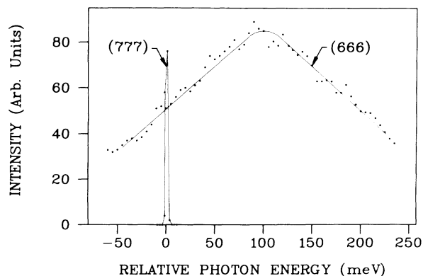
FIG. 3. Energy dependence of the scattered radiation from ^{57}\text{Fe}_2\text{O}_3 . The broad curve corresponds to the (666) reflection while the sharp curve corresponds to the (777) reflection. The continuous lines are guides for the eye.
