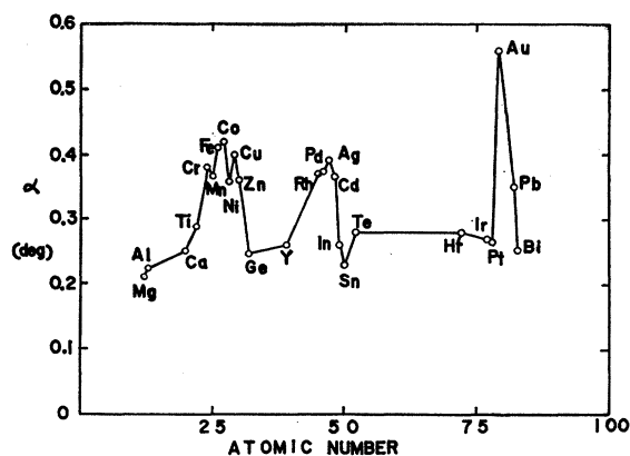
FIG. 7. Dependence of \alpha on the kind of metal.
