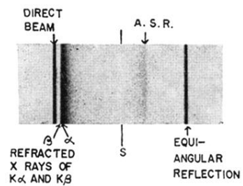
FIG. 2. Photograph of A.S.R. by a glass sample, \times 2 .
