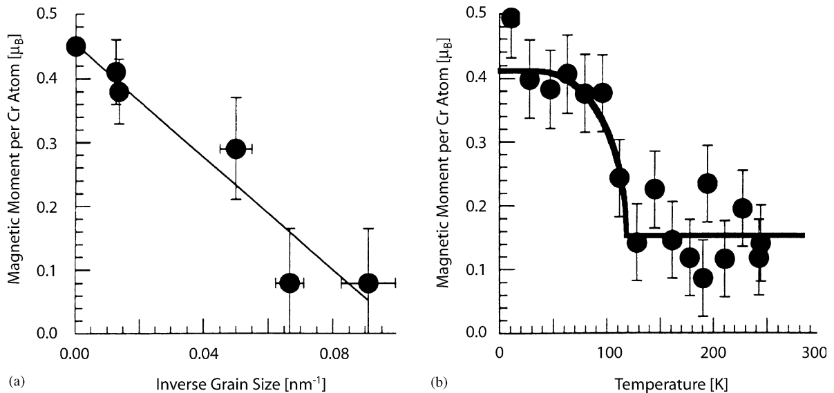
Fig. 5. (a) The magnetic moment of nanocrystalline Cr is observed to decrease with decreasing grain size. (b) The Néel point of nanocrystalline Cr with grain size of 73 nm is suppressed below T_N = 311 K observed for bulk (coarse grained) Cr. Adapted from Ref. [97].
