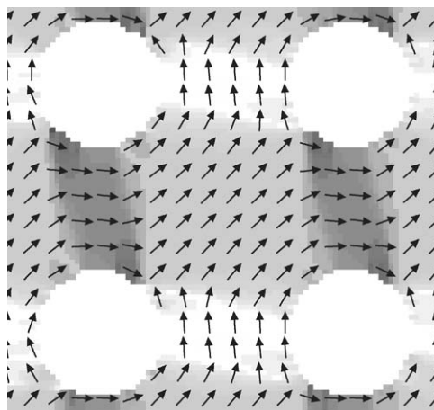
Fig. 22. A micromagnetic simulation of the spin configuration of magnetic induction in a bit constrained at the corners by four antidots (holes). Adapted from Ref. [130].
