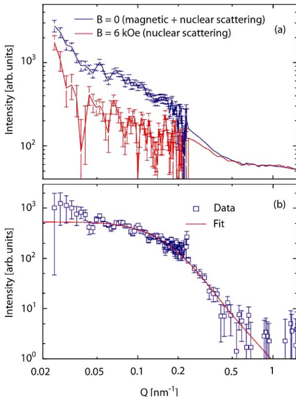
Fig. 24. Small-angle neutron scattering data from a magnetic recording disk. (a) Intensity at zero applied magnetic field and 6 kOe field. (b) Magnetic small-angle neutron scattering, which is the difference of the curves in (a). A fit to these data is shown by the line using a log-normal distribution of magnetic cluster sizes [312].
