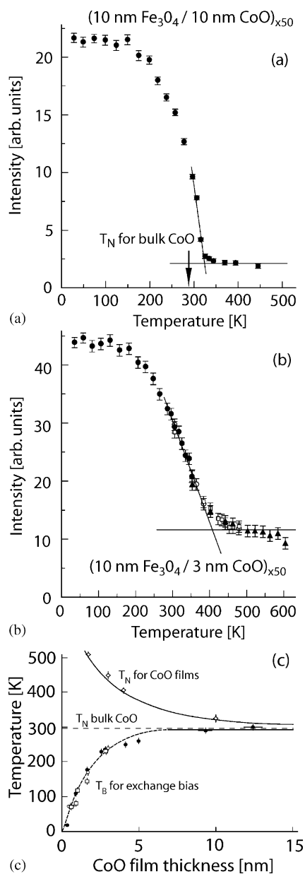
Fig. 14. The intensity of the (111) Bragg reflection as a function of temperature for a (a) (10 \text{ nm Fe}_3\text{O}_4 / 10 \text{ nm CoO})_{\times 50} and (b) (10 \text{ nm Fe}_3\text{O}_4 / 3 \text{ nm CoO})_{\times 50} multilayer. The ordering temperatures, T_N , for the CoO films deduced from data in (a) and (b) are shown in (c) as a function of film thickness. Also shown are the temperatures at which nonzero exchange bias is observed, i.e., the blocking temperatures, T_B , as determined from magnetometry.
