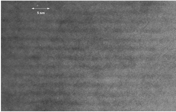
Fig. 20. A TEM micrograph of a (\text{MnSb})_{\times 1}(\text{GaSb})_{\times 6} digital superlattice (“digital alloy”) grown by atomic layer epitaxy. The Mn-containing “digital” layers are much thinner than the image indicates, because TEM is significantly more sensitive to the strain produced by the inserted atomic species than to its atomic number. Adapted from Ref. [295].
