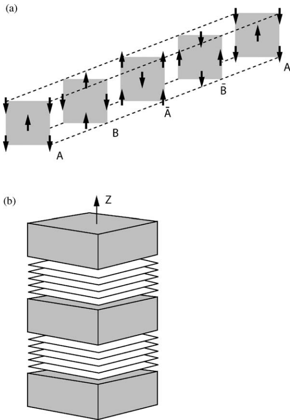
Fig. 17. (a) Schematic diagram illustrating the Type-III antiferromagnetic structure. (b) Schematic diagram showing how the antiferromagnetic planes of the Type-III structure are arranged in a superlattice.
