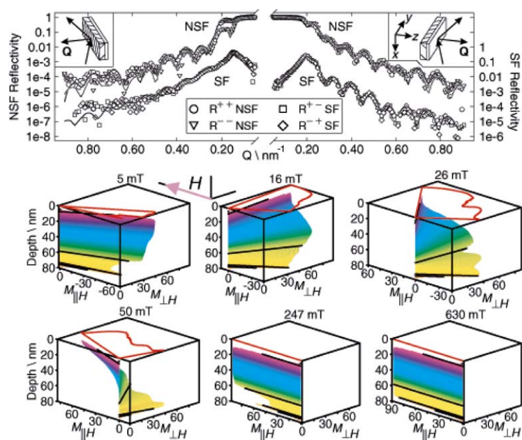
Fig. 16. (upper panel) Neutron reflectivity data taken from an exchange spring magnet. (lower panel) Schematic diagram showing the evolution of the magnetization in the soft layer at the coercive field, as deduced from neutron scattering data. Adapted from Ref. [273].
