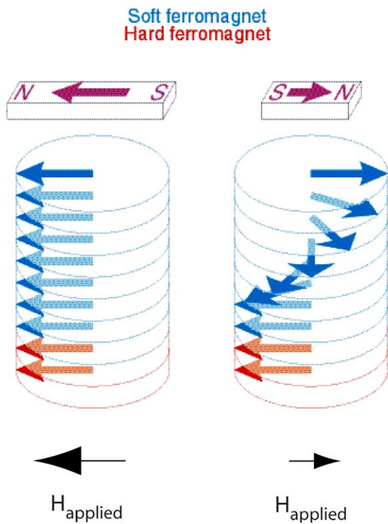
Fig. 15. The magnetization depth profile of the soft (hard) ferromagnet is shown by the blue (red) arrows. (left) The magnetizations of soft and hard ferromagnets are aligned. As the applied field is reversed and its strength increased (right), the magnetization of the soft ferromagnet begins to reverse (rotate, thus creating a “fan” magnetic structure). For the situation shown on the right, the magnetic field is not strong enough to overcome the pinning of the soft ferromagnetic layer to the hard layer (nor is the field strong enough to reverse the magnetization of the hard layer). (Figure courtesy of K. O’Donovan.)
