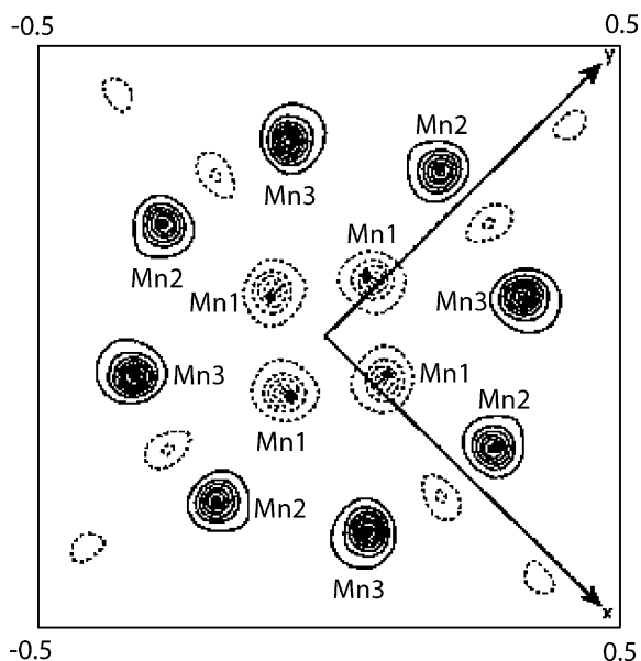
Fig. 4. A spin density map of \text{Mn}_{12} -acetate obtained using polarized neutron diffraction. Spin down density is shown as dashed lines, spin up as solid. \text{Mn}^{4+} ions are located on “Mn1” sites ( \mu = -2.34 \mu_B ), and \text{Mn}^{3+} ions are on sites “Mn2” ( \mu = +3.7 \mu_B ) and “Mn3” ( \mu = +3.8 \mu_B ). Adapted from Ref. [80].
