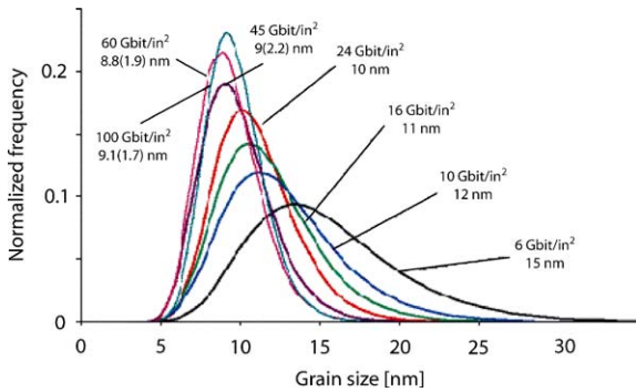
Fig. 23. Trends in grain size distributions (mean (standard deviation)) for different recording densities.
