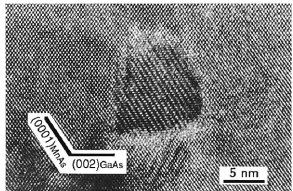
Fig. 21. High-resolution TEM image of a single-crystalline MnAs particle formed in the GaAs matrix. Adapted from Ref. [296].
