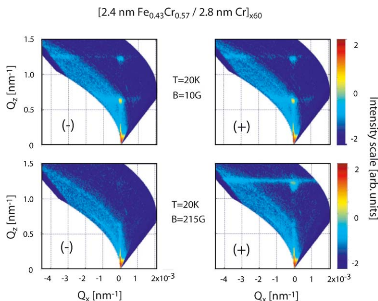
Fig. 9. Intensity map of scattering of polarized neutrons (polarization state antiparallel (–) or parallel (+) to the applied field) shown as a function of momentum transfer parallel to the sample surface ( Q_x ) and normal to the sample surface ( Q_z ). The Bragg reflection from the chemical periodicity of the superlattice ( Q_z \sim 1.2 \text{ nm}^{-1} ) is observed for both polarization states in (near) remanence (upper panels, B = 10 \text{ G} ). The half-order reflection ( Q_z \sim 0.6 \text{ nm}^{-1} ), indicative of long-range antiferromagnetic order of the Fe layer magnetization, is also observed. In saturation ( B = 215 \text{ G} , lower panels), spin-dependent scattering is observed for the superlattice reflection (indicative of ferromagnetic order). Separate values for magnetic and chemical roughness can be determined from the off-specular scattering (the streak of intensity parallel to the Q_x -axis). (Figure courtesy of H. Zabel.)
