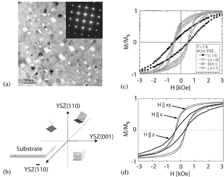
Fig. 3. (a) TEM image of \alpha -Fe particles embedded in yttria-stabilized zirconia (YSZ); diffraction spots in the inset show that the \alpha -Fe lattice is coherent with the YSZ matrix; (b) three possible and approximately equally populated orientations of \alpha -Fe in the YSZ matrix; (c) measured magnetization curves with orientations of the field normal (closed symbols) and parallel (open symbols) to the substrate surface; (d) calculated hysteresis loops for film of oriented Fe cubes with field applied normal (solid line) and parallel (dotted lines) to film plane.
