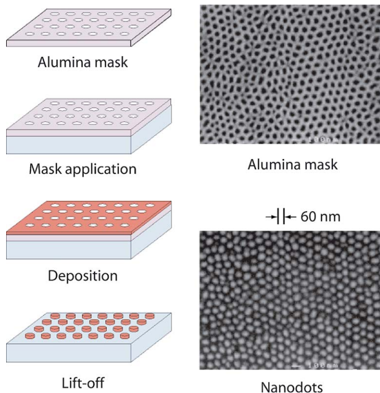
Fig. 12. Schematic diagram of an inorganic process for fabricating large areas of nanodots. An alumina mask with holes is placed on a substrate. Material is deposited through the holes, then the mask is removed, leaving \sim 60 nm diameter dots on the substrate.
