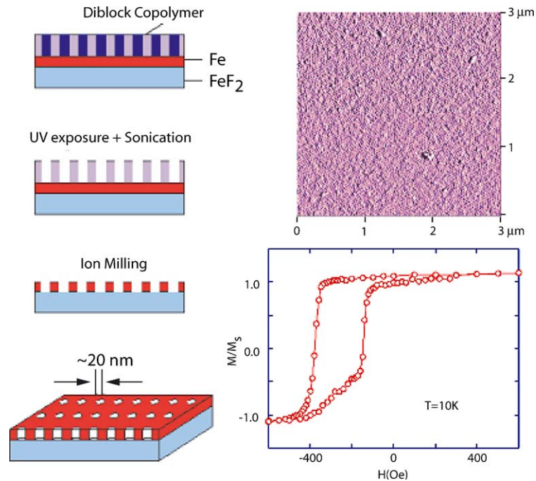
Fig. 13. Schematic diagram (left) showing a three-step process used in the fabrication of networked islands of iron metal (atomic force microscope image at upper right). The network exhibits unusual magnetic hysteresis, including exchange bias, and multiple magnetization reversal processes. Figure adapted from Ref. [207].
