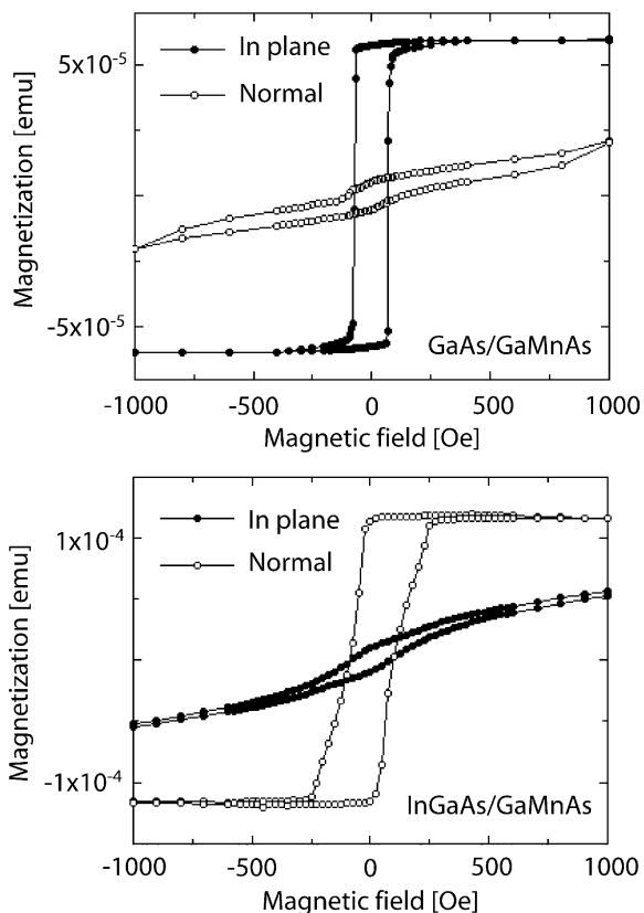
Fig. 19. Hysteresis loops for samples under compressive and tensile strain in the layer plane (upper and lower panels, respectively) at 5 K. The open and full symbols are taken with the applied magnetic field normal and parallel to the layer, respectively. Note that the easy axis is in the layer plane for compressively strained layers, and is normal to the plane for tensile strained layers [332].
