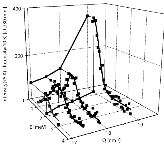
Fig. 10. Spin wave dispersion curves measured for a superlattice of Dy and Y. Adapted from Ref. [172].
