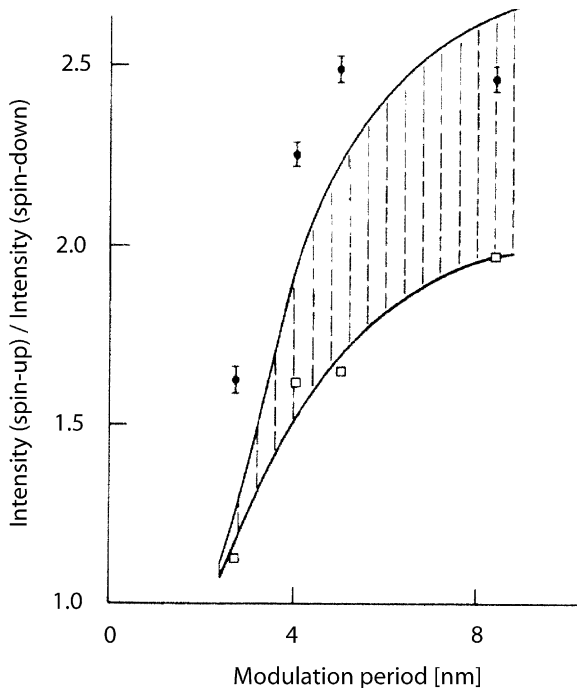
Fig. 8. Measured ratio of spin-up neutron intensity to spin-down intensity (•) plotted as a function of modulation period in the Ni/Mo superlattice. The experimental measurements are consistently larger than those calculated for a wide variety of model structures in which the magnetic roughness was constrained to be the same as the chemical roughness (as determined from X-ray scattering), indicating that the magnetic Ni/Mo interface is smoother than the chemical Ni/Mo interface. Adapted from Ref. [86].
