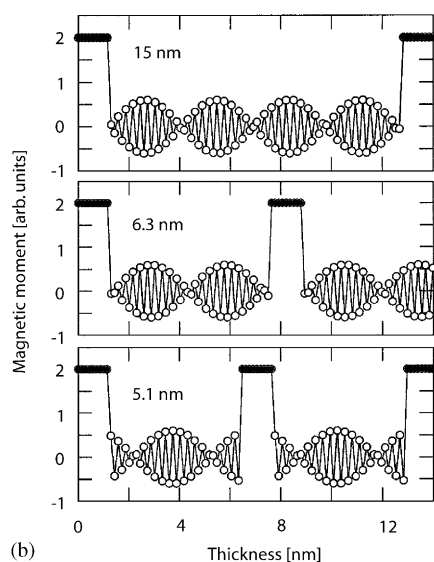
Fig. 6. (a) Temperature dependence of the antiferromagnetic Bragg reflection from thin layers of Cr in an Fe/Cr superlattice, with Fe layer thickness of 1.4 nm. From left to right in the figure, the Cr layer thicknesses, t_{Cr} , for the samples were 5.1, 6.3, 11.5 and 19 nm. Inset: The measured Néel temperatures for the Cr layers in the superlattice samples. (b) Variation of magnetic moment in the Fe and Cr layers for multilayer samples with different Cr layer thickness as deduced from neutron scattering. Adapted from Ref. [41].
